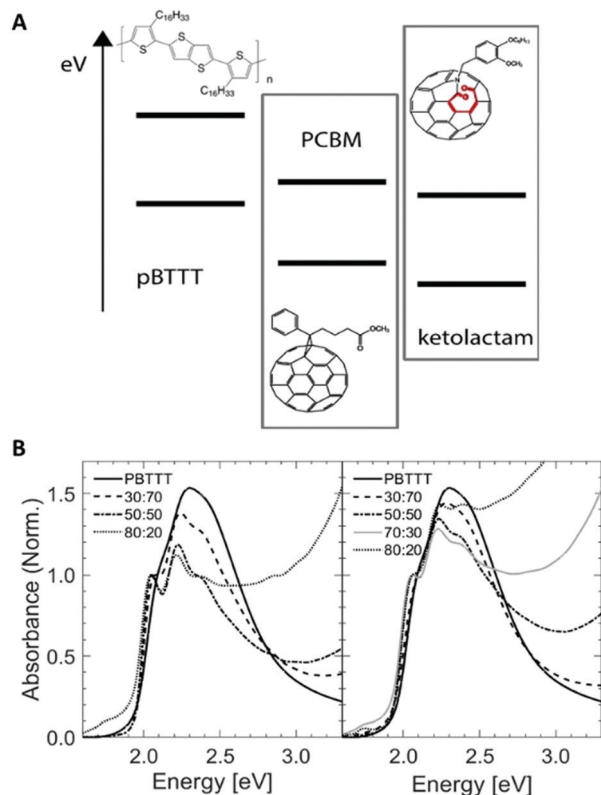
Fig. 1 (A) Schematic representation of the energy levels of the polymer (PBTtT) and fullerene acceptors, i.e., PCBM and ketolactam fullerene, used here to scrutinize the power of temperature/composition phase diagrams for property mapping of corresponding blends. Chemical structures are shown as insets. (B) UV-vis spectroscopy data of a range of blends of PCBM:PBTtT (left) and ketolactam:PBTtT (right; compositions given as mass ratio), and for comparison: neat PBTtT.
