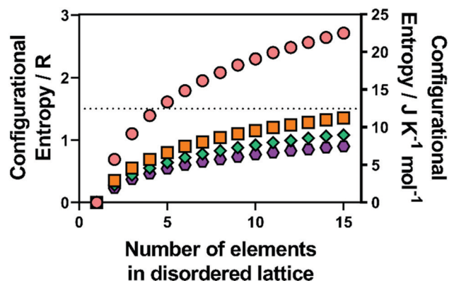
Fig. 1 Calculated configurational entropy (in both R and J K^{-1} mol^{-1} ) for species with a single disordered sub-lattice (M) for (pink circles) alloys with a single lattice, and a range of common metal chalcogenide materials with a single chalcogenide sub-lattice ( i.e. X is all O, S, Se or Te) for (orange squares) MX, (blue diamonds) M_2X_3 and (purple hexagons) MX_2 .
