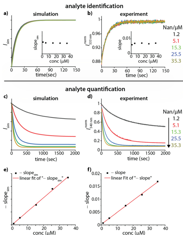
Fig. 3 (a) Simulated kinADA and (b) experimental kinADA PFO traces monitored at 533 nm ( \lambda_{\text{exc}} = 376 nm) upon varying analyte concentrations of Nan (1.2–35.3 μM) in the presence of 1 μM CB8 in water, followed by the spiked addition of MPCP indicator dye (50 μM). See Fig. S2 in ESI† for further details and parameters used for the simulations. The insets show the slope of the initial linear part of the kinetic traces for different analyte concentrations (c) Simulated kinIDA and (d) Experimental kinIDA traces monitored at 540 nm ( \lambda_{\text{exc}} = 462 nm) upon varying analyte concentrations for Nan (1.2–35.3 μM) while keeping the concentration of the CB7 ⇌ berberine complex at 1 μM. See Fig. S4 in ESI† for further details and parameters used for the simulations. (e and f) Plots of the initial slopes of the kinetic traces versus the analyte concentration. The calibration curves obtained from a linear fit are shown as a red line.
