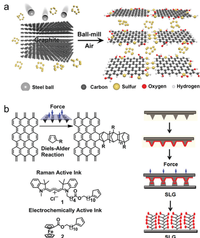
Fig. 12 (a) Schematic illustration of edge functionalization process of graphene by ball milling (reprinted with permission from ref. 458 Copyright 2014 ACS Nano). (b) Molecular structure of Diels–Alder cycloaddition reaction for mechanical force accelerated graphene functionalization (left) and schematic drawing for patterned functionalization process (right) (reprinted with permission from ref. 193 Copyright 2013 J. Am. Chem. Soc. ).
