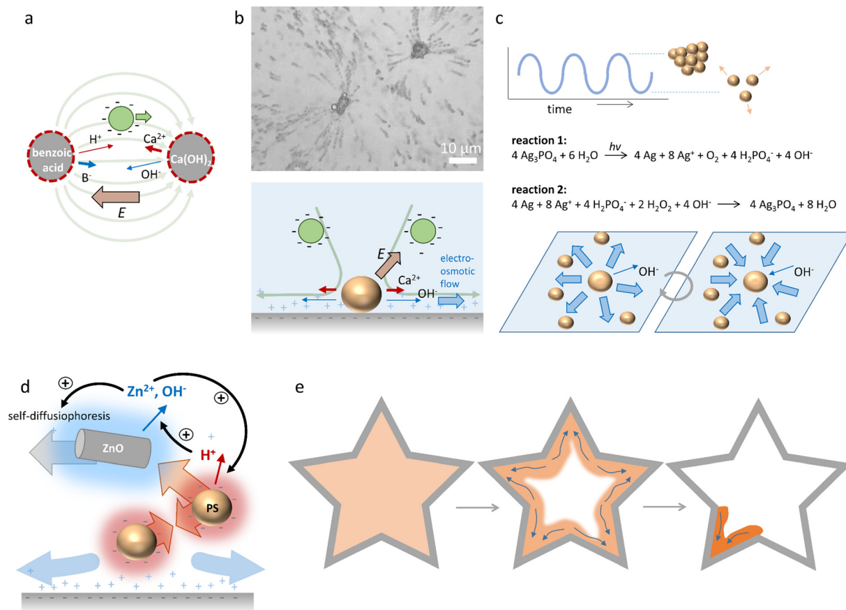
Fig. 15 Self-organisation driven by diffusiophoresis. (a) Motion pattern of negatively charged tracer particles along a sustained pH gradient between benzoic acid and \text{Ca(OH)}_2 sources. 162 (b) Electroosmotic flow drives the motion of tracer particles amongst \text{CaCO}_3 microparticles on a negatively charged substrate. Reprinted (adapted) with permission from ref. 163. Copyright 2012 American Chemical Society. (c) Oscillatory clustering and dispersion of \text{Ag}_3\text{PO}_4 microparticles in an aqueous \text{H}_2\text{O}_2 solution, where reaction (1) and (2) alternate and drive the electroosmotic flow. 170 (d) Diffusiophoretic colloidal swarms based on ZnO nanorods and sulfonated polystyrene microbeads, that are coupled via an ion exchange reaction that provide positive and negative feedback to ZnO/polystyrene clustering. (e) Collective swarm behaviour of ZnO/polystyrene particles (orange) that accumulate in the edge of the geometry (grey) with the highest curvature. 171
