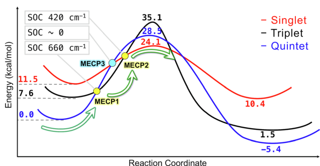
Fig. 7 Multi-state reaction mechanism for the iron-catalyzed C(sp 2 )–H bond activation involving three different spin states. The energies are obtained with the ωB97X-V/def2-TZVP//B3LYP-D3(BJ)/def2-SVP level of theory. The bold blue, black and red numbers are relative energies in kcal mol −1 with respect to the quintet reactant energy. The values of spin–orbit coupling between the spin states at MECPs are shown in gray boxes.
