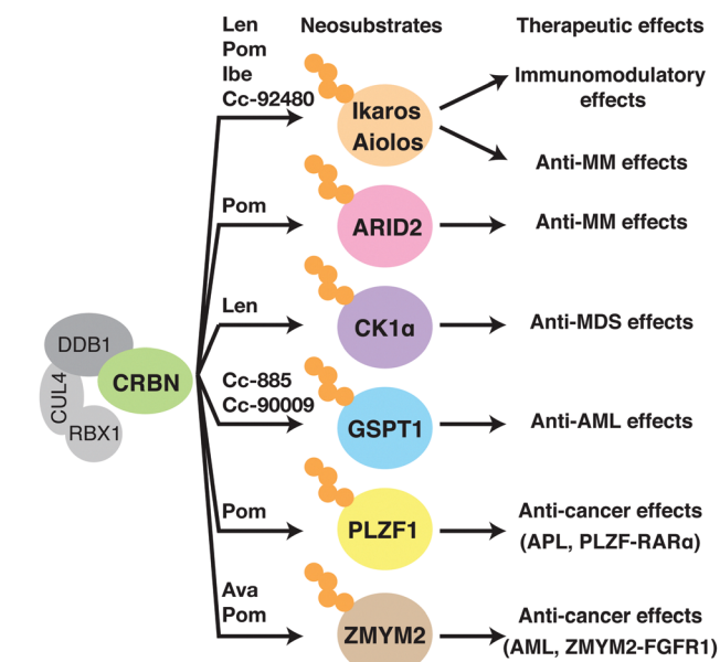
Fig. 5 Mechanisms of therapeutic effects of thalidomide-based glue degraders. Binding of thalidomide-based glue degraders to CRBN induces degradation of corresponding neosubstrates, resulting in the therapeutic effects shown in the figure. Abbreviations: len, lenalidomide; Pom, pomalidomide; Ava, avadomide; Ibe, iberdomide; MM, multiple myeloma; MDS, myelodysplastic syndromes; AML, acute myeloid leukemia; APL, acute promyelocytic leukemia.
