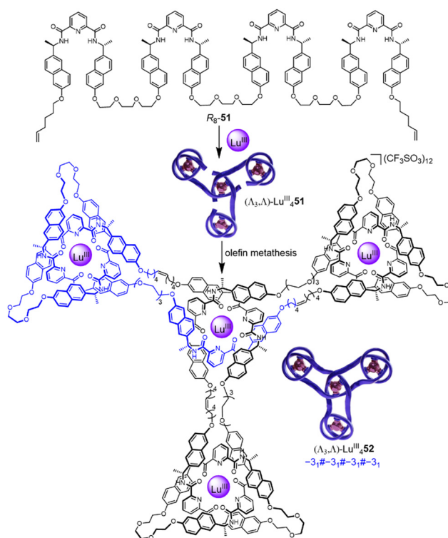
Fig. 18 Synthesis of triskelion knot (\Lambda_3, \Lambda)\text{-Lu}_4^{\text{III}}\text{52} by Vernier template synthesis. 27
