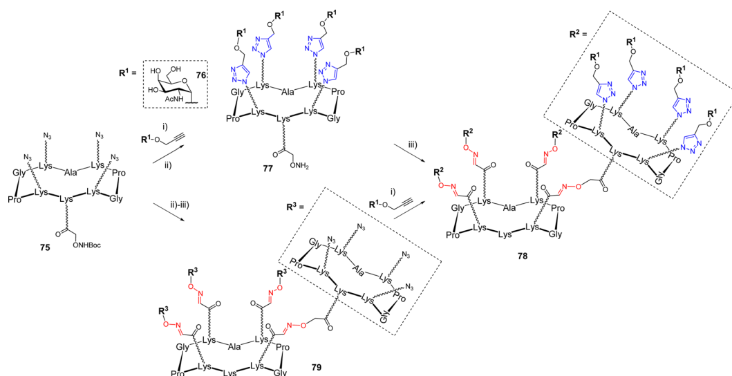
Scheme 15 Convergent synthesis of the hexadeca-azide glycodendrimer 78 by CuAAC/OL. Reagents and conditions: (i) CuSO 4 ·5H 2 O, THPTA, sodium ascorbate, DMF/PBS buffer (pH 7.5) (1 : 1), r.t., 2 h, 70% (divergent synthesis); (ii) TFA/H 2 O (6 : 4), r.t., 1 h, 77% over two steps for 77 ; (iii) 51 , 0.1% TFA in H 2 O, 37 °C, 45 min, 90% for 78 ; 85% for 79 .
