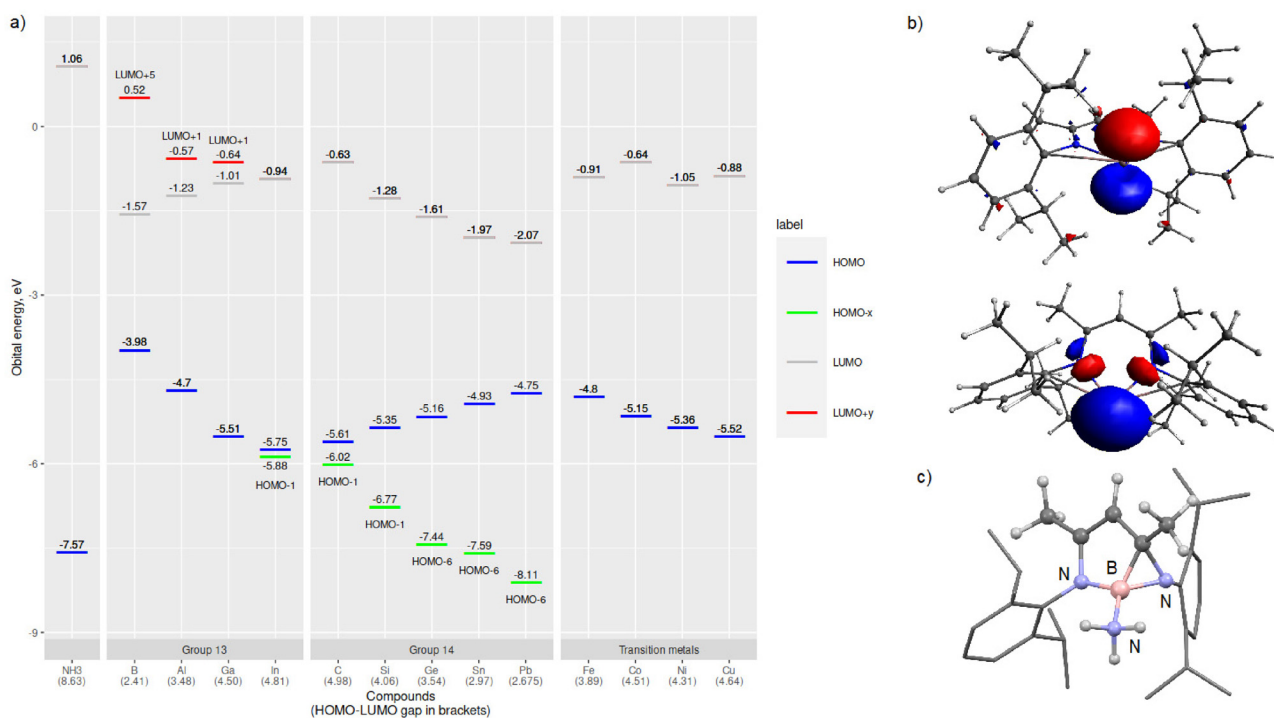
Fig. 2 (a) Calculated HOMO- x and LUMO+ y energy levels for the computed LM/L'M species. HOMO- x indicates a lone pair MO and LUMO+ y an empty p-orbital associated with the main group element M, (b) LUMO+1 (upper) and HOMO (lower) of LGa (isovalue set at \pm 0.05 a.u.), and (c) structure of the rearranged LB-NH 3 , Dipp-groups are shown as a wireframe format for clarity.
