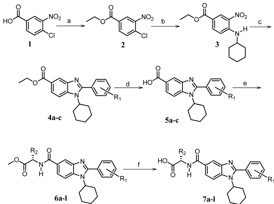
Scheme 1 Synthetic strategy for the benzimidazole mono-peptides ( 7a-l ). a Reagents and conditions: (a) EtOH, conc. \text{H}_2\text{SO}_4 (catalytic), reflux; (b) cyclohexylamine (2.5 equiv.), TEA (3.0 equiv.), THF, r.t.; (c) substituted benzaldehyde (1 equiv.), \text{Na}_2\text{S}_2\text{O}_4 (3 equiv.), DMSO, 90 °C; (d) NaOH (1.1 equiv.), water, reflux; (e) amino acid methyl ester hydrochloride (1 equiv.), NMM (2.5 equiv.), TBTU (1.25 equiv.), DMF, r.t.; (f) \text{LiOH} \cdot \text{H}_2\text{O} (1 equiv.), water : THF (2 : 1), 0 °C. \text{R}_1 = 4\text{-F} , 4\text{-OCH}_3 , 2\text{-Cl} -6-F; \text{R}_2 = \text{CH}_3 , \text{CH}(\text{CH}_3)_2 , \text{CH}_2\text{-CH}(\text{CH}_3)_2 , 3-indolylmethyl. * Further for the substitution pattern see Table 1.
