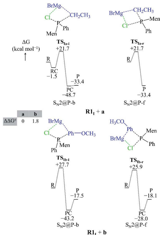
Fig. 4 Geometries of the TSs and PESs of the R1 I + a and R1 I + b S_N2@P reactions in THF. The bond lengths/distances are in Å. The \Delta G and \Delta\Delta G^\ddagger are in kcal mol -1 .
