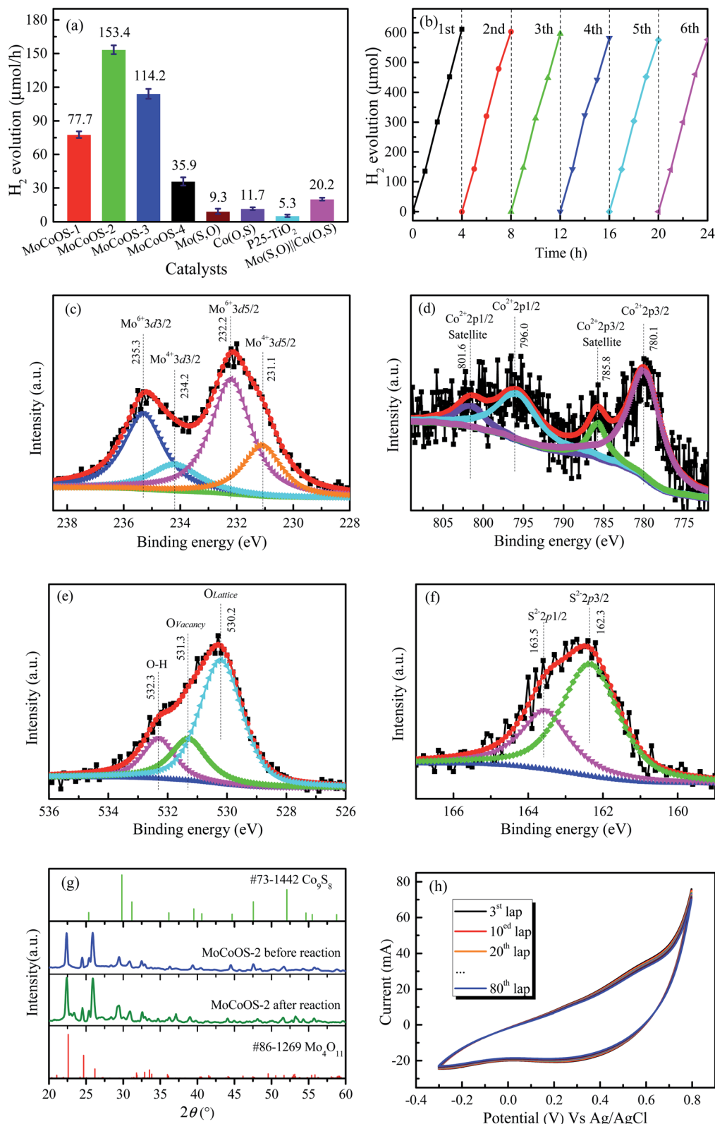
Fig. 7 (a) Hydrogen production of MoCoOS, Mo(S 2 O), Co(O,S), Mo(S 2 O)@Co(O,S) and P25-TiO 2 catalysts. (b) Recycling hydrogen production reaction performance of MoCoOS-2. (c-f) XPS spectra of MoCoOS-2 after the hydrogen evolution reaction. (g) XRD patterns of MoCoOS-2 before and after the hydrogen evolution reaction. (h) Cyclic voltammetry of MoCoOS-2 for 80 cycles.
