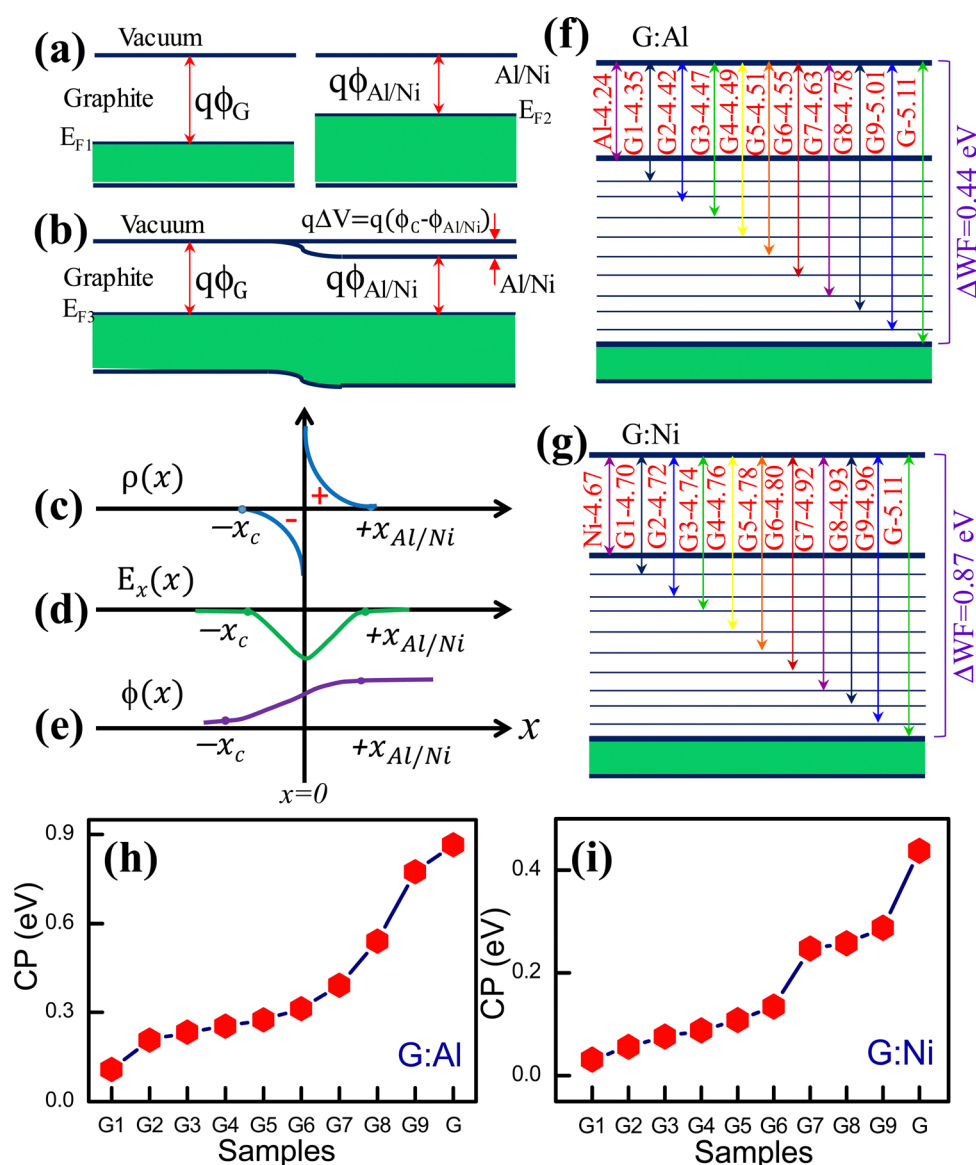
Fig. 2 Graphite–Al/Ni composites (a) before and (b) after junction formation. (c) Space charge density distribution, (d) electric field distribution, (c) charge density distribution and (d) electric field, (e) electric potential at the junction. WF of various composite (f) G:Al and (g) G:Ni electrodes and the contact potential (CP) of (h) G:Al and (i) G:Ni electrodes.
