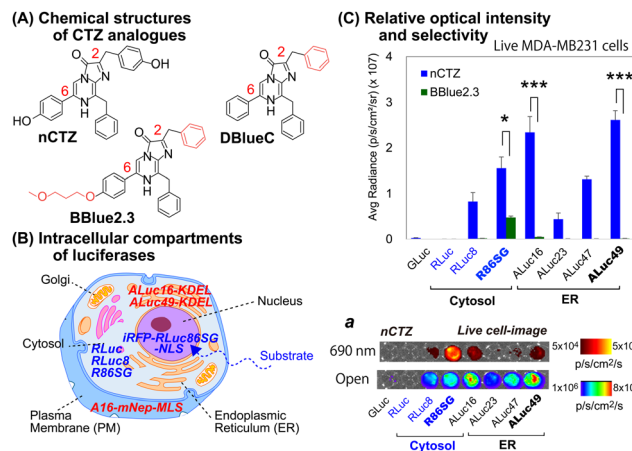
Fig. 1 (A) The chemical structures of native coelenterazine (nCTZ) and its analogues (DBBlueC and BBlue2.3) used in this study. The CTZ analogues diffuse into the intracellular compartments and react with the expressed marine luciferases. (B) Schematic illustration of a mammalian cell showing the location specific distribution of expressed marine luciferases. Each luciferase is designed to be sequestered into a distinctive cellular compartment, i.e., the cytosol, nucleus, plasma membrane (PM), or endoplasmic reticulum (ER). (C) The quantitative results of live cells that are selectively bright according to the substrates and luciferases used for the study. The absolute BL intensities were independently measured in triplicate from a single experiment ( n = 3 ). The p -values (student t test) are *** \leq 0.001 , ** \leq 0.01 , and * \leq 0.05 . Inset 'a' shows the representative BL images of Fig. 1(C), where the BL images were obtained in an open channel or with a 690 nm bandpass filter.
