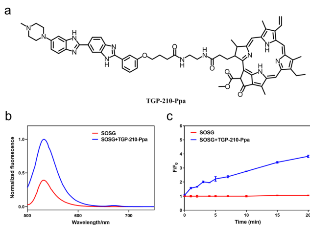
Fig. 1 (a) Chemical structure of TGP-210-Ppa . (b) Fluorescence spectra of TGP-210-Ppa after irradiation with 670 nm light (70 mW cm -2 ) for 5 min. (c) The increase of SOSG fluorescence at 530 nm after incubation with TGP-210-Ppa and irradiation by 670 nm light (70 mW cm -2 ) for 0–20 min. λ ex = 488 nm. Data are shown as mean ± SEM (n = 3).
