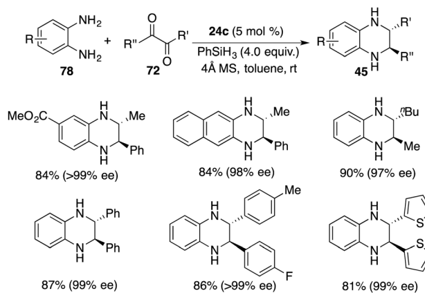
Scheme 43 Enantio- and diastereoselective synthesis of trans -2,3-disubstituted 1,2,3,4-tetrahydroquinoxalines.
