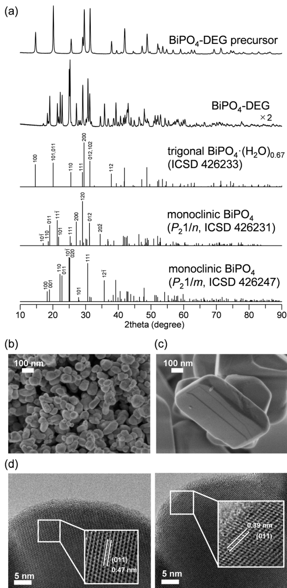
Fig. 2 (a) XRD patterns for BiPO 4 -DEG precursor, BiPO 4 -DEG, trigonal BiPO 4 ·(H 2 O) 0.67 (ICSD 426233), monoclinic BiPO 4 ( P 2 1 / n , ICSD 426231), and monoclinic BiPO 4 ( P 2 1 / m , ICSD 426247). SEM images for (b) BiPO 4 -DEG and (c) BiPO 4 -HT. (d) TEM images for BiPO 4 -DEG.
