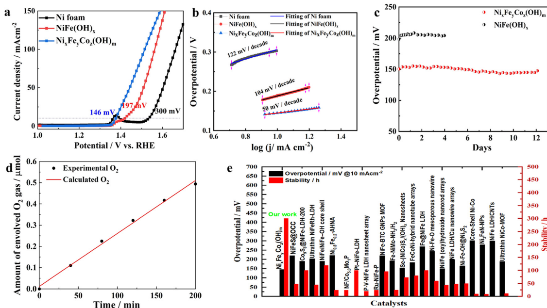
Fig. 2 OER performance. (a) Polarisation curves after IR-compensation and (b) corresponding Tafel plots of the NF, \text{NiFe}(\text{OH})_x and \text{Ni}_x\text{Fe}_y\text{Co}_z(\text{OH})_m electrodes in 1 M KOH. (c) Long-term stability tests at a constant current density of 10 \text{mA cm}^{-2} for the \text{NiFe}(\text{OH})_x and \text{Ni}_x\text{Fe}_y\text{Co}_z(\text{OH})_m electrodes in 1 M KOH. (d) \text{O}_2 amounts detected by gas chromatography (dark dots) and the calculated amounts of \text{O}_2 (red line) by \text{Ni}_x\text{Fe}_y\text{Co}_z(\text{OH})_m catalyst. The measurement was performed at j_{\text{OER}} = 10 \text{ mA cm}^{-2} in 1 M KOH. (e) Comparison of this work and reported overpotential required to achieve current densities of 10 \text{mA cm}^{-2} and the related stability for various catalysts in 1 M KOH. RHE stands for reversible hydrogen electrode.
