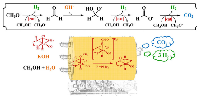
Fig. 8 The mechanism of \text{RuHCl(CO)(HN(C}_2\text{H}_4\text{PPr}_2)_2\text{)} catalyzed methanol dehydrogenation. 268 Reproduced with permission from ref. 268. Copyright (2016) American Chemical Society.
