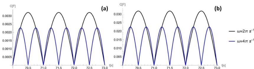
Fig. 8 Capacitance generated over time at the frequency of 2\pi \text{ s}^{-1} (black) and 4\pi \text{ s}^{-1} (blue) for a porous electrode. The pore size r is 10^{-5} m for (a) and 10^{-7} m for (b). Parameters used are: \bar{C} = 5 \times 10^{-2} \text{ F m}^{-2} ; S_T = 0.002 \text{ m}^2 ; \varepsilon = 0.5 ; \theta_w = 131.18^\circ ; V_{\text{ref}} = 1.5 \text{ V} ; \eta = 6.3 \times 10^{-2} \text{ Pa s}^{-1} ; and \gamma = 2.27 \times 10^{-2} \text{ N m}^{-1} .
