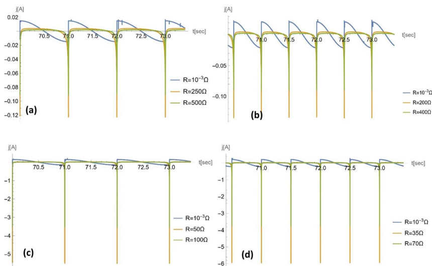
Fig. 9 Temporal profile of the electrical current for a porous electrode. For a pore size of r_p = 10^{-5} m, the frequency used is (a) \omega = 2\pi \text{ s}^{-1} and (b) \omega = 4\pi \text{ s}^{-1} ; for a pore size of r_p = 10^{-7} m, the frequency used is (c) \omega = 2\pi \text{ s}^{-1} and (d) \omega = 4\pi \text{ s}^{-1} . For each plot, 3 different loads were chosen on the basis of: (1) near-zero value, which shows a temporal profile consistent with the literature with consideration of no/negligible load; 23 (2) resistance at which the power reaches maximum; and (3) resistance larger than that corresponding to the maximum power. Other parameters used are: V_{\text{ref}} = 1.5 \text{ V} , \bar{C} = 5 \times 10^{-2} \text{ F m}^{-2} ; S_T = 0.002 \text{ m}^2 ; \varepsilon = 0.5 ; \theta_w = 131.18^\circ ; \eta = 6.3 \times 10^{-2} \text{ Pa s}^{-1} ; and \gamma = 2.27 \times 10^{-2} \text{ N m}^{-1} .
