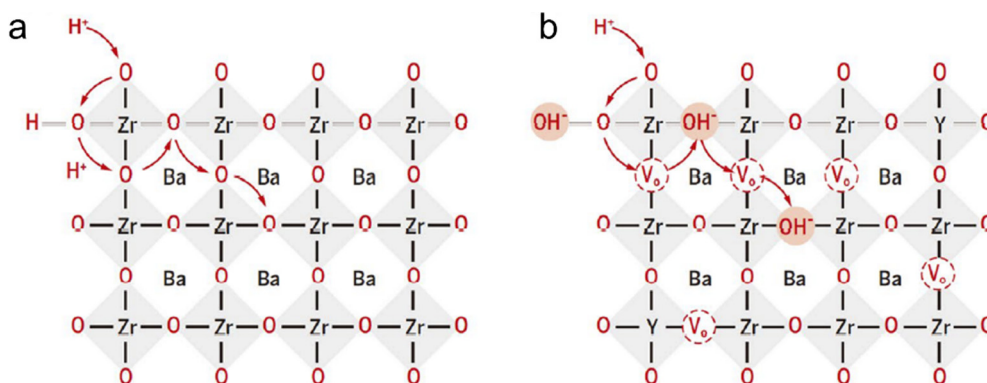
Fig. 2 Schematics of two \text{H}^+ conducting mechanisms in a \text{BaZrO}_3 -based perovskite oxide: (a) the Grotthuss mechanism and (b) the vehicle mechanism. 17
