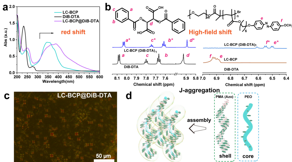
Fig. 3 (a) UV spectra and (b) Locally amplified ^1\text{H} NMR spectra of LC-BCP, DiB-DTA, and LC-BCP@DiB-DTA with a molar ratio of 1. (c) POM picture of LC-BCP@DiB-DTA at 90 ^{\circ}\text{C} . (d) Schematic diagram of the formation of the hierarchical helical structure.
