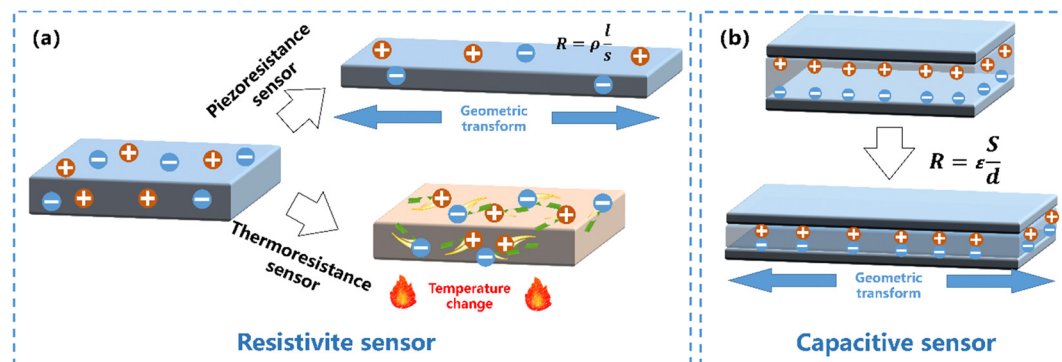
Fig. 9 Schematic illustration of the structure and working mechanism of a (a) resistive sensor, and (b) a capacitive sensor.
