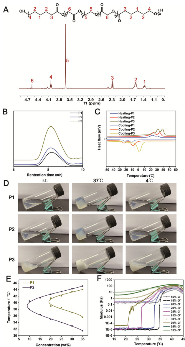
Fig. 2 (A) 1 H NMR spectrum of P2. (B) GPC curves of P1, P2 and P3. (C) DSC thermograms of P1, P2 and P3 at a heating or cooling rate of 20 °C min -1 . (D) Photographs of P1, P2, and P3 solutions at different temperatures with a polymer concentration of 30% (wt%). (E) Phase diagram of P1 and P2 solutions with different concentrations in a water bath plotted by a vial inversion method at different temperatures. (F) Storage modulus G' and loss modulus G'' of P2 solutions with different concentrations as a function of temperature.
