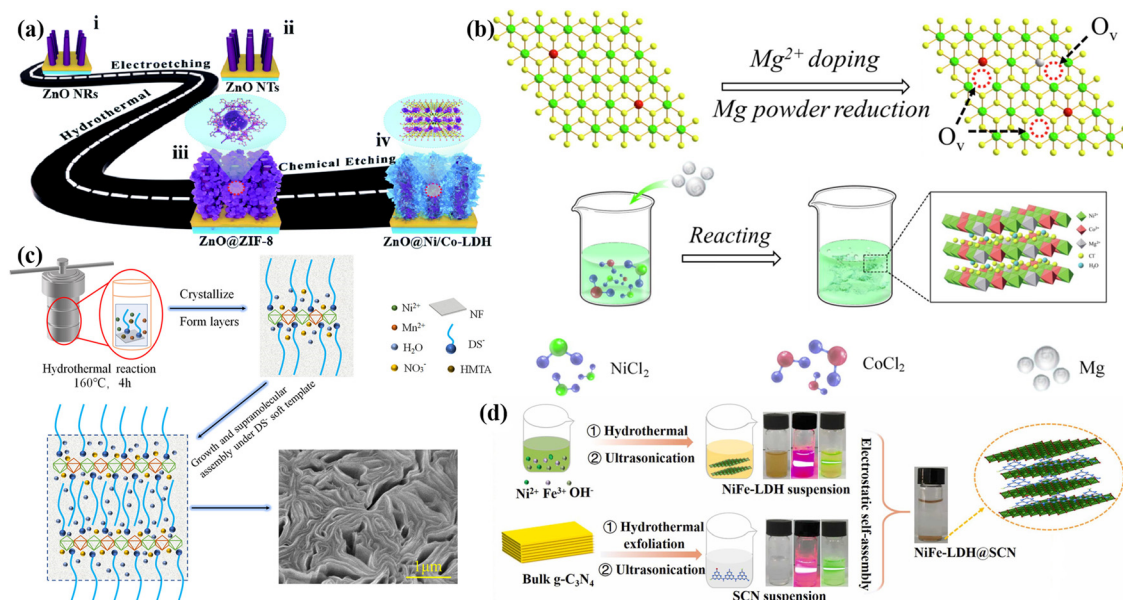
Fig. 14 (a) Synthesis scheme of the ZnO@Ni/Co-LDH film. Adapted with permission from ref. 216 Copyright 2022, Royal Society of Chemistry. (b) Schematic illustration of the fabrication strategy of oxygen-vacancy abundant CoNiMg-LDHs. Adapted with permission from ref. 217 Copyright 2021, Elsevier Inc. (c) Growth mechanism of LDH with SDS as a soft template. Adapted with permission from ref. 218 Copyright 2022, Elsevier Ltd. (d) The synthetic process of the NiFe-LDH@SCN. Adapted with permission from ref. 219 Copyright 2022, Elsevier B.V.
