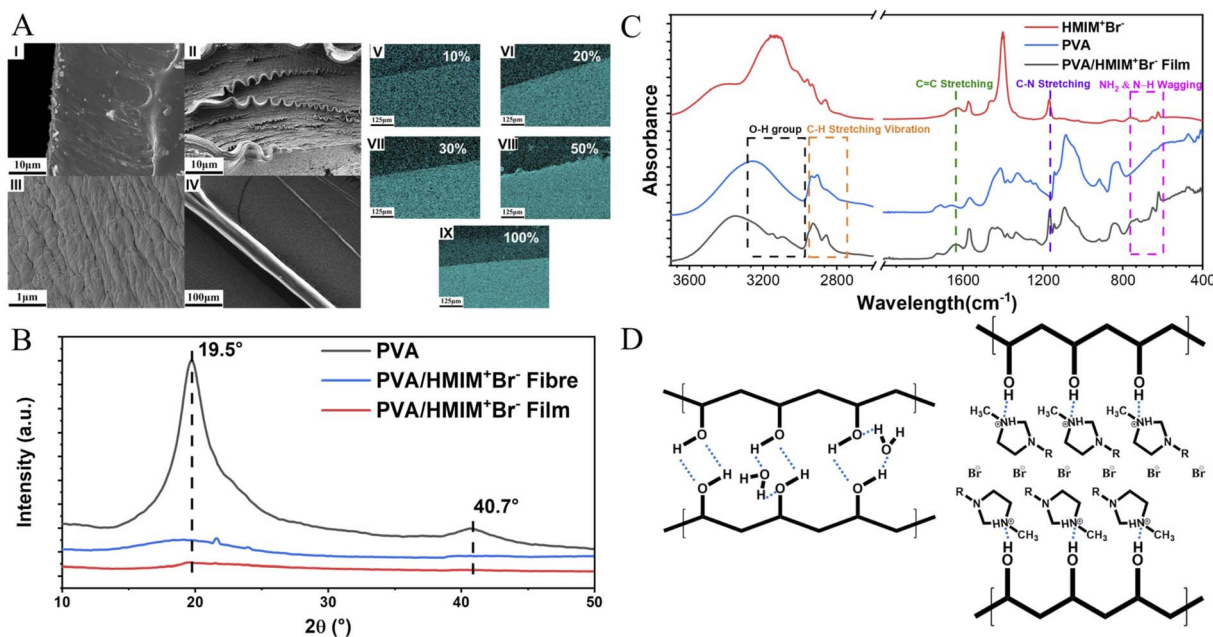
Fig. 2 (A) SEM images of the cross-section area of (I) PVA film, (II and III) PVA/Br-IL film with 10 \mu\text{m} (II) and 1 \mu\text{m} (III) scale bar, and (IV) PVA/Br-IL fibre, and (V–IX) EDX images of PVA/Br-IL film with different concentrations of [HMIM] + Br - , with bromide in green. (B) X-ray diffraction patterns of PVA and PVA/Br-IL fibre and film. (C) FTIR spectra of [HMIM] + Br - , PVA and the PVA/Br-IL film. (D) Schematic illustration of possible intermolecular interactions involved in PVA/Br-IL film formation.
