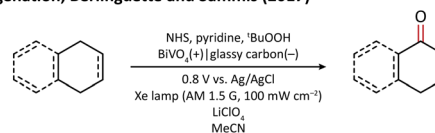
A. C–H oxygenation, Berlinguette and Sammis (2017)
