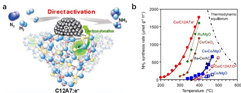
Fig. 8 (a) Reaction mechanism for \text{NH}_3 synthesis on Co/C12A7:e - catalyst. (b) Temperature dependence of \text{NH}_3 synthesis rate for the supported Co catalysts. Reaction conditions: WHSV, 18 000 mL g -1 h -1 ; pressure, 0.1 MPa. Copyright 2019, American Chemical Society.
