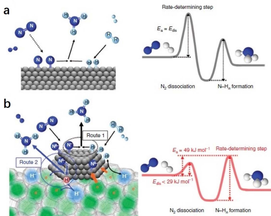
Fig. 7 Reaction mechanism and energy diagram for \text{NH}_3 synthesis on (a) conventional catalyst and (b) Ru/C12A7:e - catalyst. Copyright 2015, Springer Nature.
