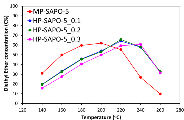
Fig. 5 Showing the DEE intermediate concentration of the reaction output for catalytic ethanol dehydration. Reaction conditions: 25 mL min -1 of nitrogen carrier gas, 10 \mu L min -1 flow of 10% heptane in ethanol, 0.3 g of catalyst sieved between 500–300 \mu m.
