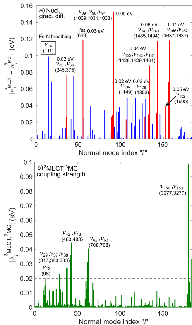
Fig. 6 Analysis of vibronic effects for the lowest four 3 MLCT and three 3 MC states of [Fe(bmip) 2 ] 2+ at the FC geometry. (a) Largest absolute difference of nuclear gradients ( |k_i^{3\text{MLCT}} - k_i^{3\text{MC}}| ) for all normal modes. For each mode, the 3 MLCT- 3 MC component leading to the largest absolute difference is selected. Absolute differences above 0.02 eV originating from a significant k_i^{3\text{MLCT}} > 0.02 eV value are highlighted in red. The numbers in eV next to mode labels are the absolute values of the largest 3 MLCT gradient components. (b) 3 MLCT- 3 MC coupling strengths ( |\lambda_i^{3\text{MLCT}, 3\text{MC}}| ) for all normal modes. For each mode, the 3 MLCT- 3 MC component leading to the largest coupling strength is selected. In parentheses, the frequency of the most important modes is given (in \text{cm}^{-1} , for both panels).
