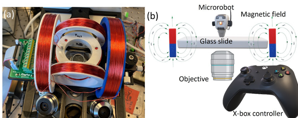
Fig. 1 Magnetic setup for the microrobot control. (a) Helmholtz coils mounted on an inverted microscope and (b) a schematic of microrobotic control employed in this study.
