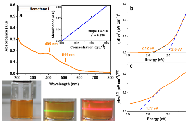
Fig. 2 Hematene I: (a) UV-Vis spectrum in water dispersion. (b) Tauc plot diagram for direct and (c) indirect transitions. Photos of Hematene I in water as a subject of the Tyndall effect with a green and red laser beam.
