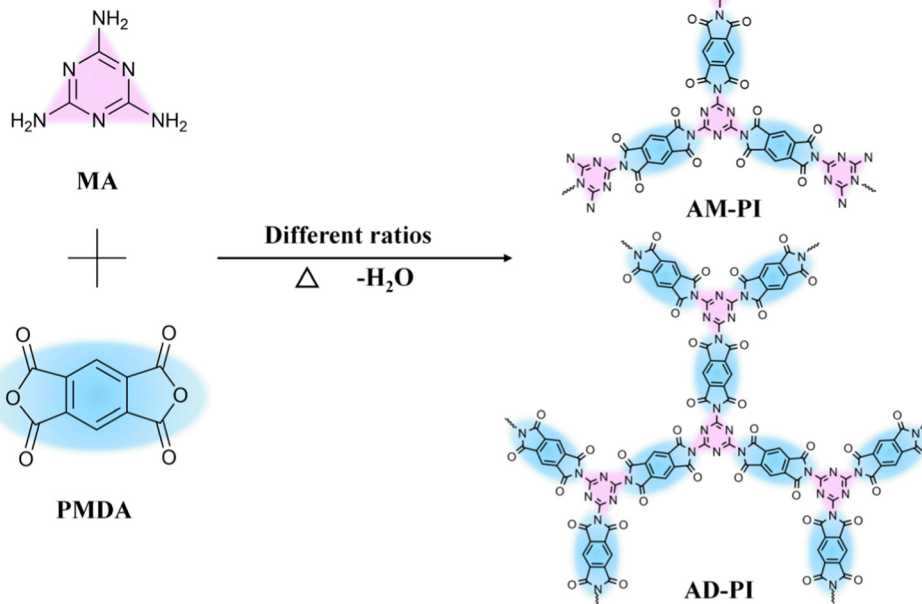
Scheme 1 Reaction scheme for the synthesis of AM-PI and AD-PI .
