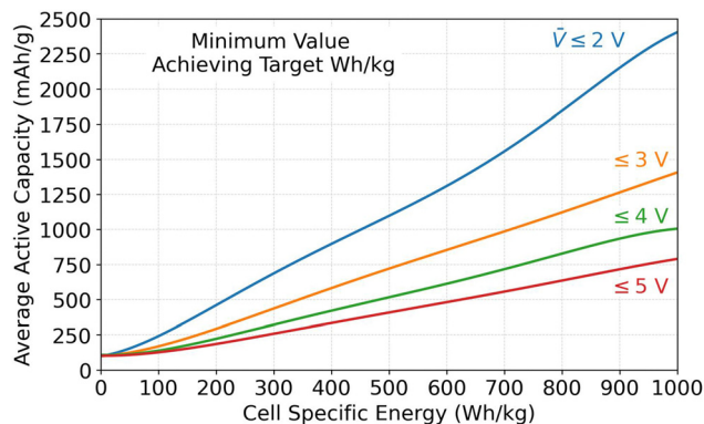
Fig. 4 Minimum average specific capacity ( i.e. , average of Q_{+, \text{act}} and Q_{-, \text{act}} ) capable of achieving specific energy targets ( \text{W h kg}^{-1} ), based on results in the Monte Carlo simulation database. Each line represents a different maximum allowable average open circuit voltage ( \bar{V} ).
