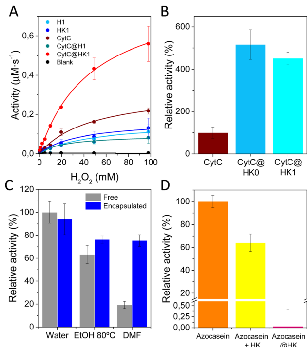
Fig. 5 (A) Kinetic analysis of the free CytC, encapsulated CytC and CytC + MOFs physical mixtures. (B) Relative activity of CytC@HK0 and CytC@HK1 biocomposites ( \text{H}_2\text{O}_2 3.27 mM). (C) Lysolytic activity retained by encapsulated Ly after exposure to different conditions. (D) Proteolysis of free azocasein, azocasein and HKUST-1 physical mixture, and encapsulated azocasein after treatment with protease.
