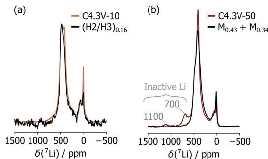
Fig. 4 (a) Comparison of the ^7\text{Li} NMR spectrum collected on C4.3V-10 and the first cycle spectrum for (\text{H}_2/\text{H}_3)_{0.16} . (b) Comparison of the ^7\text{Li} NMR spectrum collected on C4.3V-50 with the sum of spectra acquired on \text{M}_{0.43} and \text{M}_{0.34} . The spectra collected on the \text{M}_{0.43} and \text{M}_{0.34} were scaled \text{M}_{0.43} : \text{M}_{0.34} = 1 : 3.8 .
