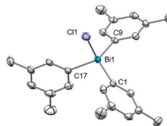
Fig. 3 Solid state structure of 10. Ellipsoids are drawn at the 50% probability level. H atoms and \text{BAR}^{\text{F}} are omitted for clarity. Selected bond lengths (Å) and angles ( ^\circ ): \text{Bi1}-\text{Cl1} : 2.4028(8), \text{Bi1}-\text{C1} : 2.185(3), \text{Bi1}-\text{C9} : 2.180(3), \text{Bi1}-\text{C17} : 2.189(3), \text{C1}-\text{Bi1}-\text{C9} : 121.63(11) , \text{C1}-\text{Bi1}-\text{C17} : 111.32(10) , \text{C9}-\text{Bi1}-\text{C17} : 112.55(11) .
