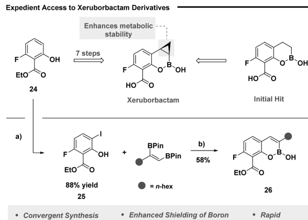
Fig. 2 Expedient access to xeruborbactam derivatives. (a) 24 (1 equiv.), 12 (1 equiv.), TIOAc (1 equiv.), DCM, rt. (b) 25 (1 equiv.), 2 (1.5 equiv.), PdCl 2 dppf-DCM (2 mol%), K 3 PO 4 (3 equiv.), MeCN/H 2 O (1:1), 60 °C.
