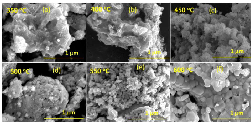
Fig. 4 Scanning electron microscope image of BiFeO 3 nanoparticles annealed at T Calcination (a) 350 °C, (b) 400 °C, (c) 450 °C, (d) 500 °C, (e) 550 °C, and (f) 600 °C.
