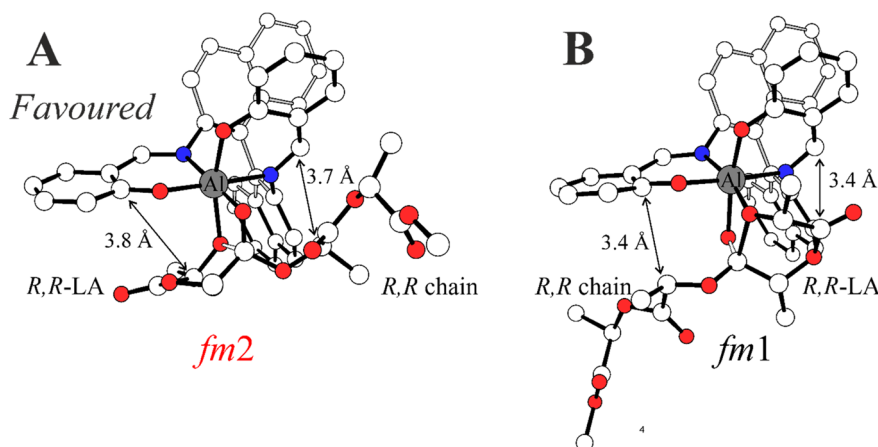
Fig. 2 Optimized DFT geometries for the RLS of RR propagation promoted by (R)-1 corresponding to the ring opening step (TS2). The energetic preference of the fm2 wrapping mode (A) with respect to fm1 (B) is due to lower steric interactions reported with arrows. Oxygen and nitrogen atoms in red and blue. Distances in Å and H atoms omitted for clarity.
