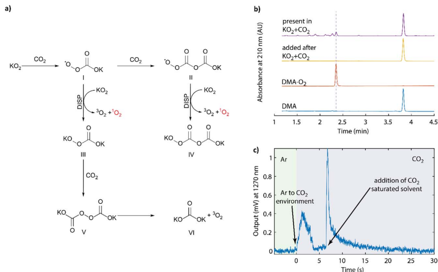
Fig. 4 (a) Reaction sequence upon reacting superoxide with \text{CO}_2 as initially described by Sawyer. 64 The final DISP step forming \text{}^1\text{O}_2 was identified in this work. (b) HPLC elugram of DMA exposed to asymmetric \text{K}_2\text{C}_2\text{O}_6 (yellow trace) and DMA present during the reaction of \text{KO}_2 and \text{CO}_2 (purple trace). (c) NIR output signal around 1270 nm during the reaction of \text{KO}_2 with \text{CO}_2 . The \text{KO}_2 and 50 mM 18-crown-6 suspension in \text{CH}_3\text{CN} was initially kept under Ar, then the headspace was purged by \text{CO}_2 , and then \text{CO}_2 -saturated \text{CH}_3\text{CN} was added.
