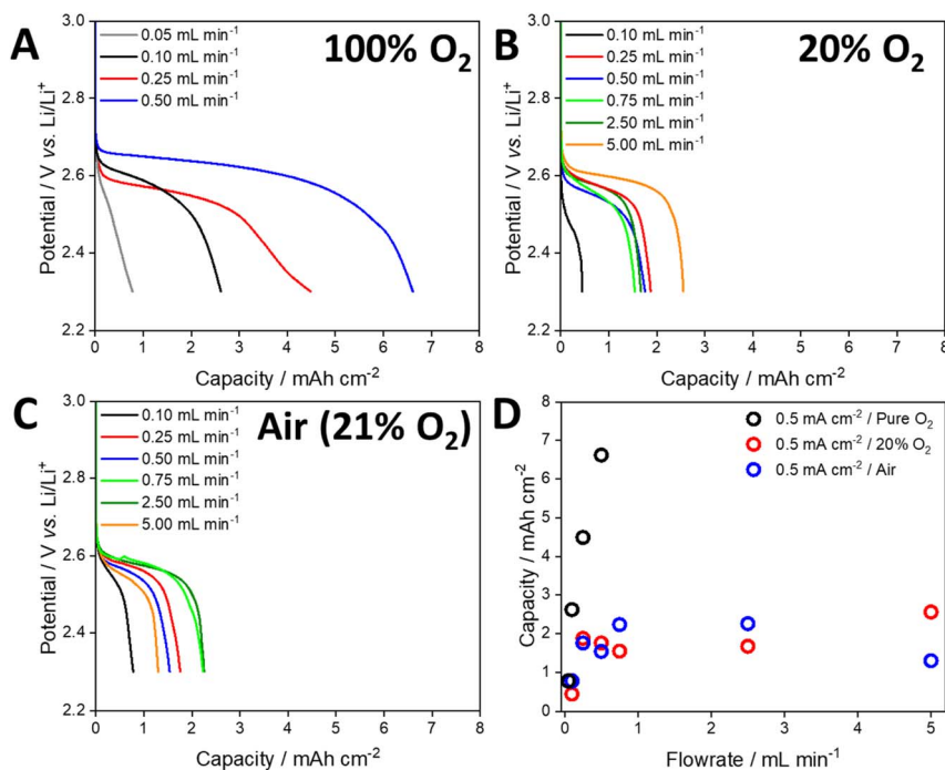
Fig. 3 Discharge profiles of cells discharged at a current density of 0.5 \text{ mA cm}^{-2} under a flow of (A) 100% \text{O}_2 , (B) 20% \text{O}_2 with \text{N}_2 balance and (C) air. (D) Shows the areal capacity of these cells.
