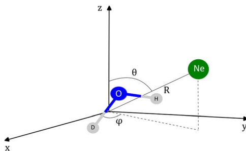
Fig. 4 Coordinates employed in the description of the HOD + Ne system. The origin of the coordinate system corresponds to the center of mass of the HOD molecule.
