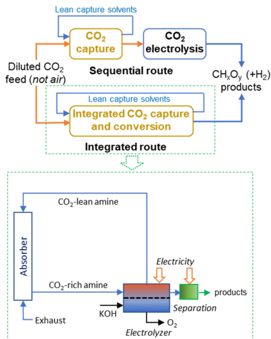
Fig. 2 Simplified block diagrams of sequential and integrated routes for amine-based \text{CO}_2 capture and electrolysis with a more detailed scheme for the integrated \text{CO}_2 capture and direct \text{CO}_2 electroreduction from the capture medium. Some elements, such as the compression unit between the stripper and the electrolyser, are not shown.
