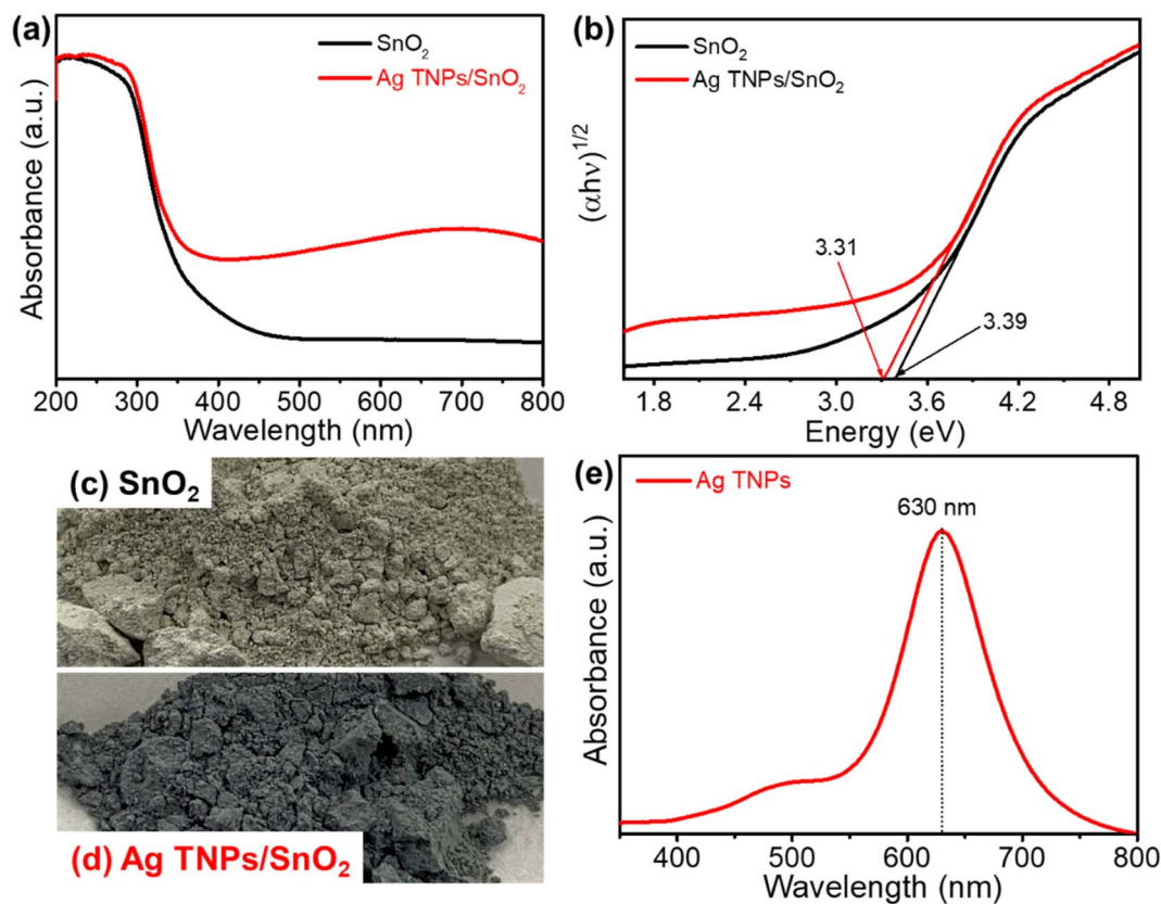
Fig. 3 (a) UV-Vis DRS and (b) Tauc plots of \text{SnO}_2 and Ag TNPs/ \text{SnO}_2 ; (c and d) optical images of as-prepared \text{SnO}_2 and Ag TNPs/ \text{SnO}_2 ; (e) UV-Vis absorption spectrum of Ag TNPs.
