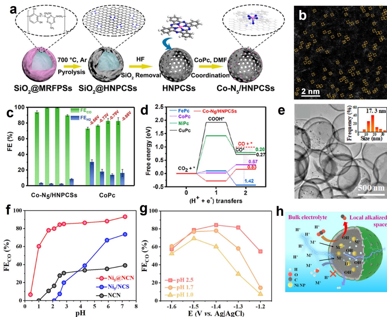
Fig. 6 (a) Synthesis procedures and (b) magnified HAADF-STEM image of hollow N-doped porous carbon spheres with single-atom \text{Co-N}_5 sites ( \text{Co-N}_5\text{/HNPCSSs} ). (c) Faradaic efficiencies for \text{CO} and \text{H}_2 production at the given potentials over \text{Co-N}_5\text{/HNPCSSs} and \text{CoPc} . (d) Calculated \text{eCO}_2\text{RR} free energy profiles of \text{Co-N}_5\text{/HNPCSSs} catalyst and \text{MPc} ( \text{M} = \text{Co}, \text{Fe}, \text{Ni}, \text{Cu} ). Reproduced with permission from ref. 114. Copyright 2018, American Chemical Society. (e) TEM image of \text{Ni NPs@N-doped carbon nanocages} ( \text{Ni@NCN} ). The inset shows the metal NPs size distribution. (f) \text{FE}_{\text{CO}} and (g) current density of the best-performing \text{Ni@NCN} sample in acidic electrolyte condition. (h) Schematic diagram of the pH environment and ions transportation around the \text{Ni@NCN} catalyst. Reproduced with permission from ref. 46. Copyright 2022, American Chemical Society.
