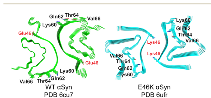
Fig. 1 Cryo-EM structures of WT (green) and E46K (cyan) \alpha Syn fibrils. The most discriminating residues Gln62, Thr64, and Val66 project outward in PDB 6cu7 but inward in PDB 6ufr. E46 and K46 are buried in each structure.
