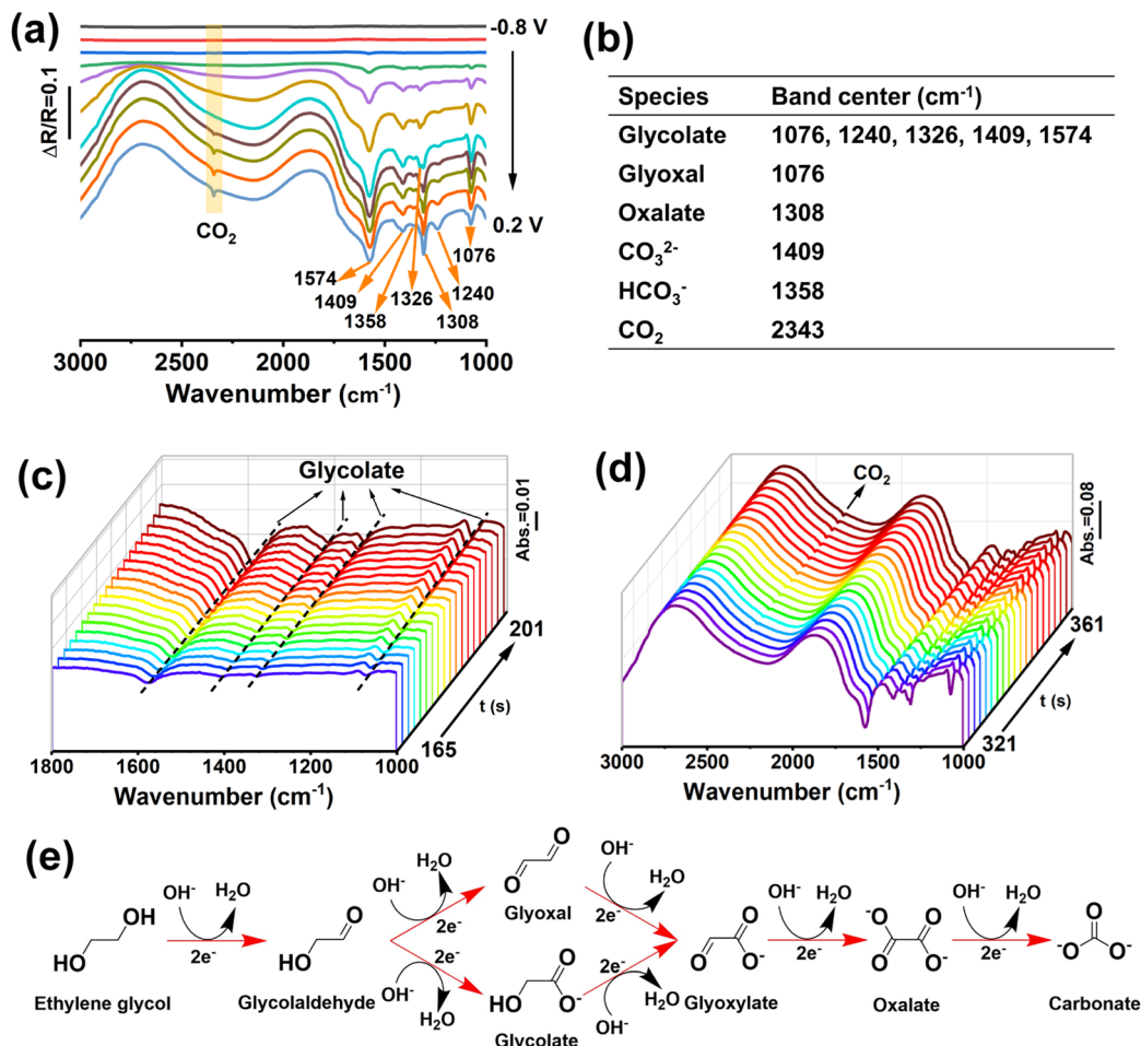
Fig. 4 (a) In situ FTIR spectra of M-PtBiMo IMSSs in 1 M KOH + 1 M EG. (b) IR bands and their assignment for the EGOR. Real-time in situ FTIR spectra of M-PtBiMo IMSSs at (c) -0.5 V and (d) -0.1 V, with an interval of 2 s. (e) Schematic of the proposed reaction pathways for the EGOR at the M-PtBiMo IMSSs in alkaline media.
