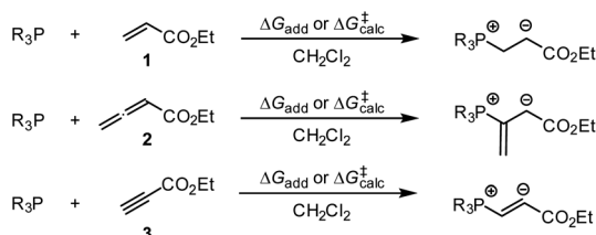
Scheme 6 Gibbs activation ( \Delta G_{\text{calc}}^\ddagger ) and reaction energies ( \Delta G_{\text{add}} ) of \text{PR}_3 additions to Michael acceptors 1–3 .
